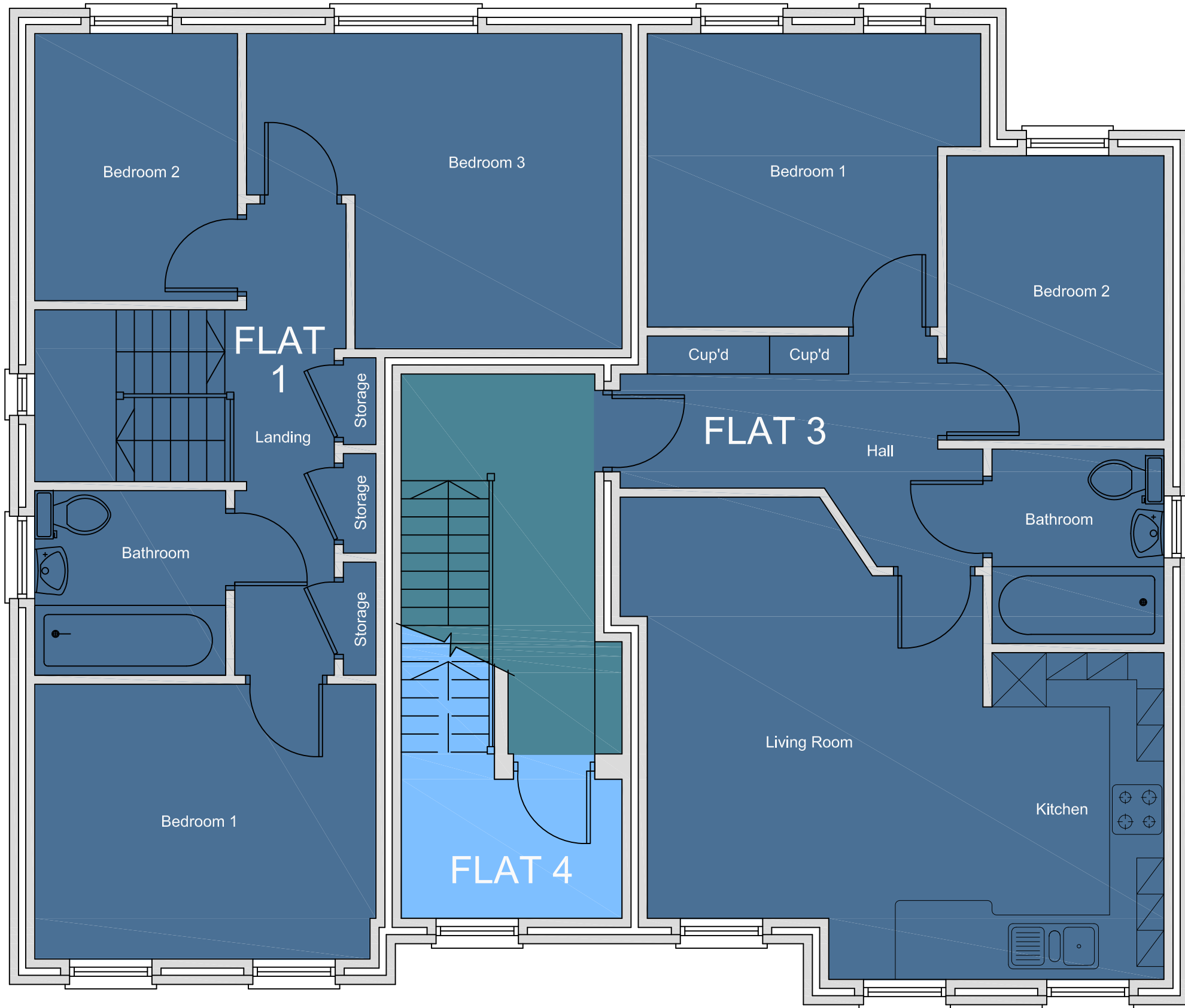
FLAT 4 First Floor Plan
